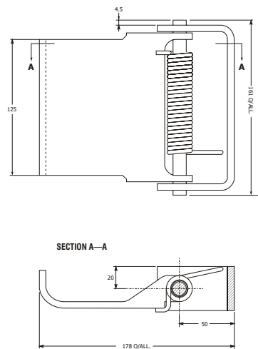
1. 92CW050801 Latch Assembly
