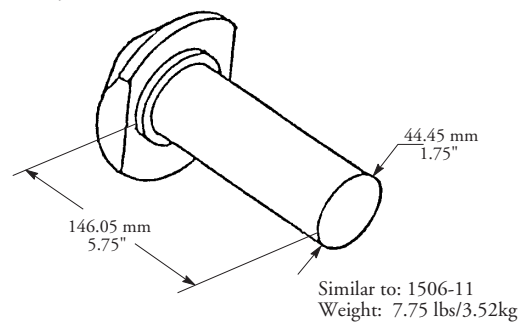
Part No.: 15-11
