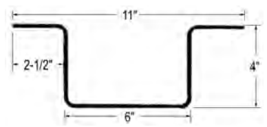
PINES 11" Crossmember
