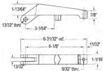
1. PEN25-05
