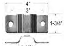
1. FRUDCF2138-1 Guide back plate
