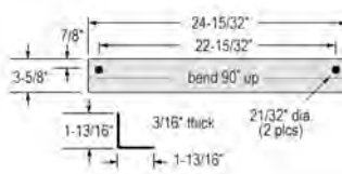
1. WAB13S00542 Brace
