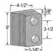
1. FRUWCA0015
