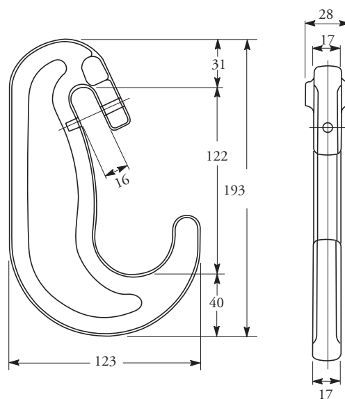
1. 56 ML-5030 Eye Hook
