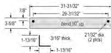
1. WAB13S00543 Brace
