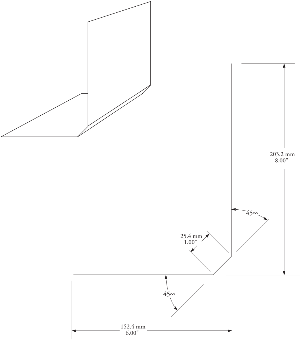
1. 53RFANG6X7AD Air Deflector Length: 96" (2438.4 mm) Thickness: 0.25" (6.35 mm) & 0.1875" (4.76 mm) Material: Aluminum
