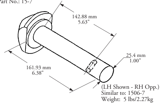
Part No.: 15-7
