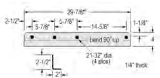
1. WAB13S00402 Brace
