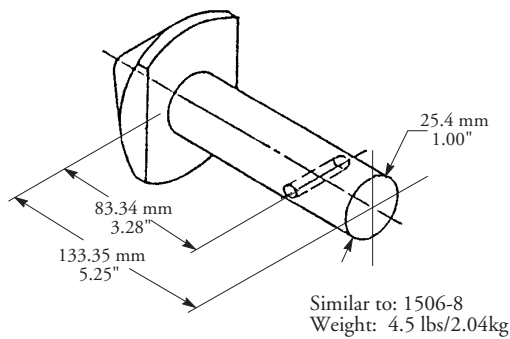
Part No.: 15-8
