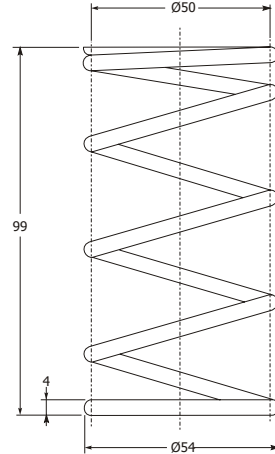
1. 924471 Compression Spring
