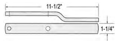
Door Latch Handle
