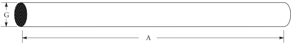
1. 53RFANG6X7AD Air Deflector Length: 96" (2438.4 mm) Thickness: 0.25" (6.35 mm) & 0.1875" (4.76 mm) Material: Aluminum
