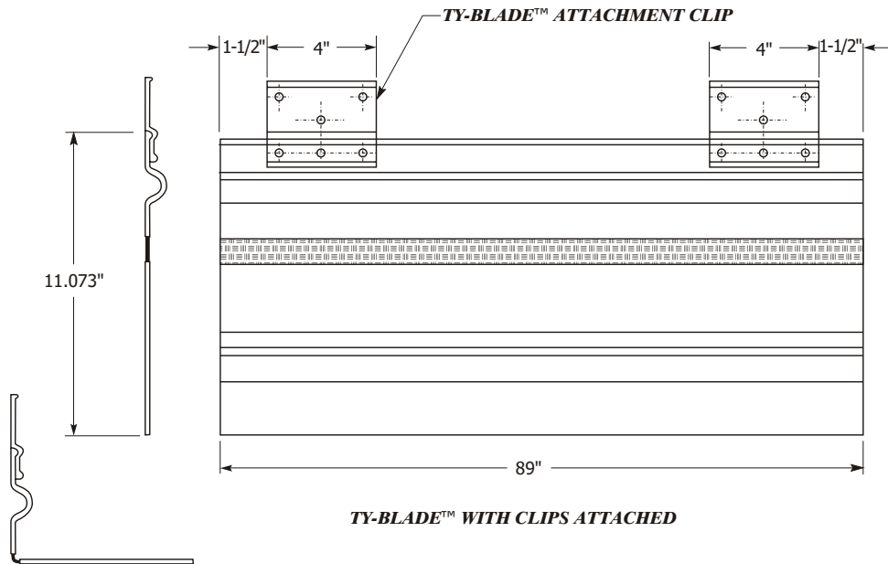
1. 73RFFNITB897 Ty-Blade
