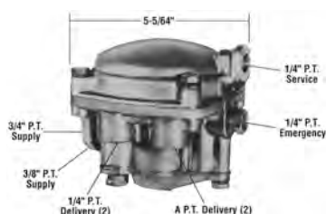
RE-6 Relay Emergency Valve
