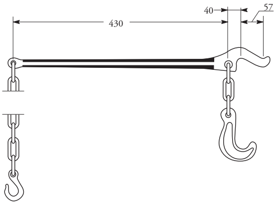
1. 56 ML-5140 11 mm Tensioner
