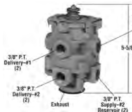
Dual Brake Valve
