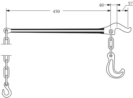
1. 56 ML-5150 13 mm Tensioner
