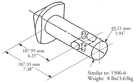
Part No.: 15-6
