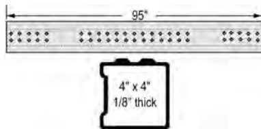
Steel Pooched Bumper Tube
