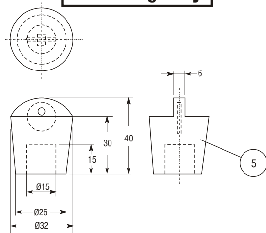
1. 40RF1948102 Drain Plug Assy.
