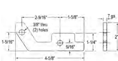
1. PEN25-05
